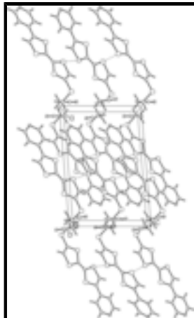
Fig. 2. The crystal packing diagram view along the crystallographic b -axis.
